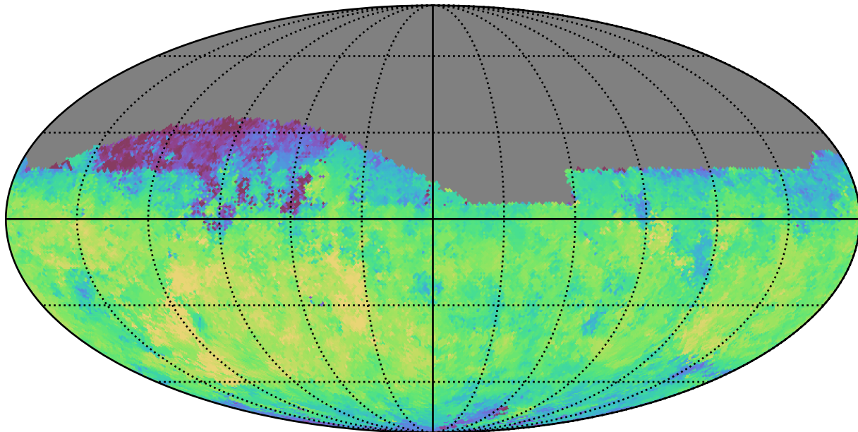
noroll_v3.4_10yrs Yr 1 i band: Median fiveSigmaDepth
