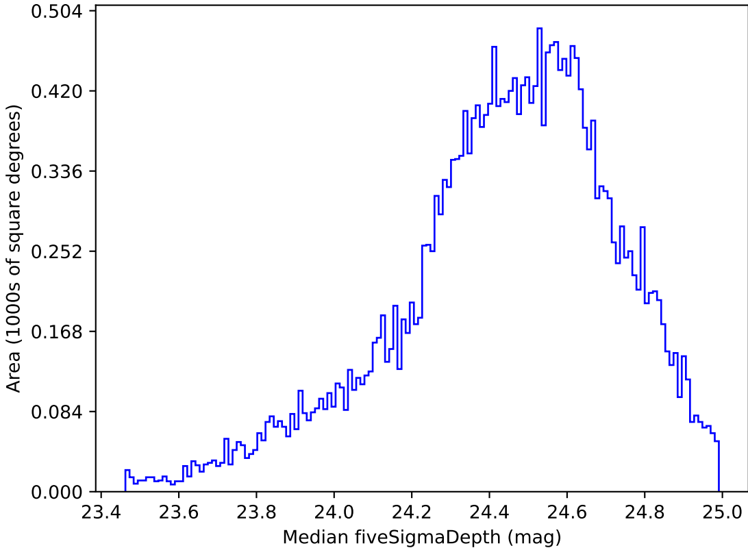
noroll_v3.4_10yrs Yr 1 g band: Median fiveSigmaDepth
