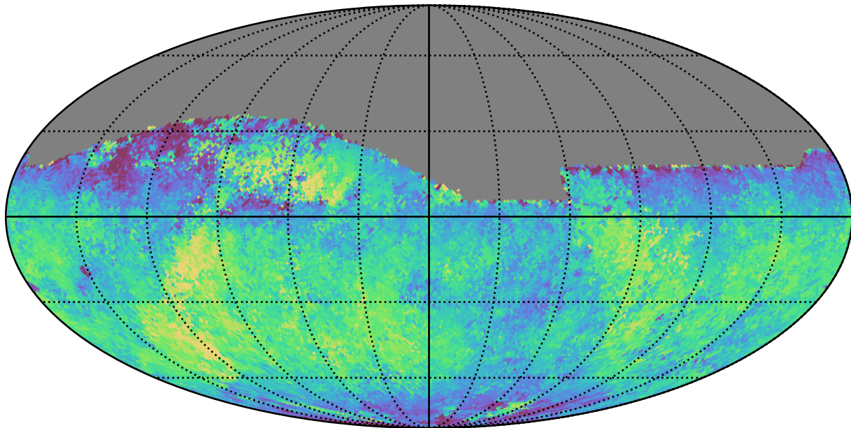
noroll_v3.4_10yrs Yr 1 all bands: Median fiveSigmaDepth
