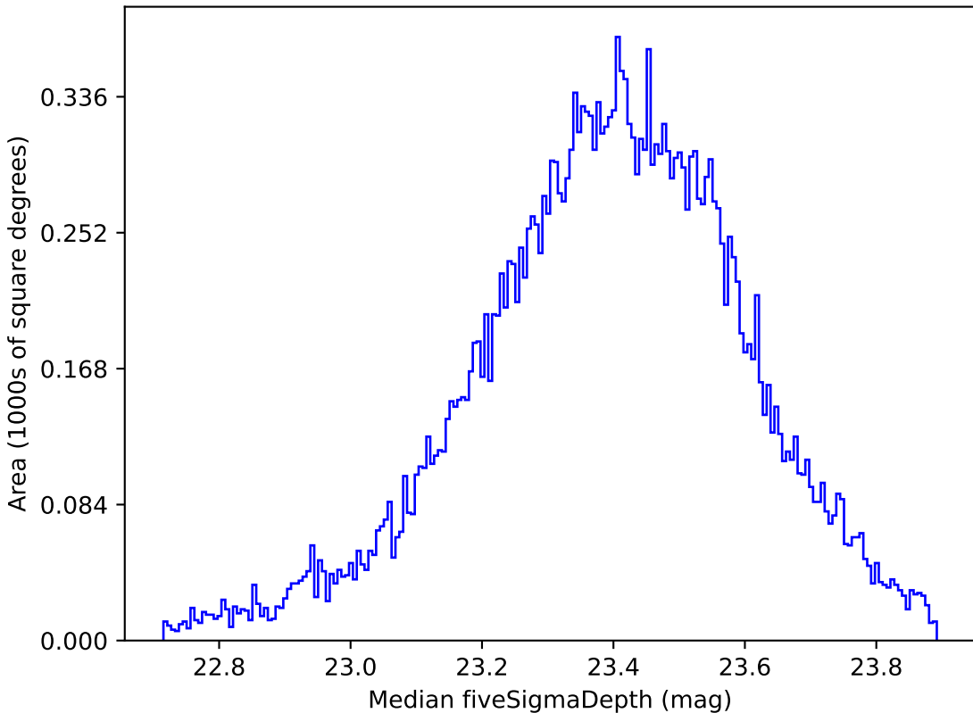
noroll_v3.4_10yrs Yr 1 all bands: Median fiveSigmaDepth
