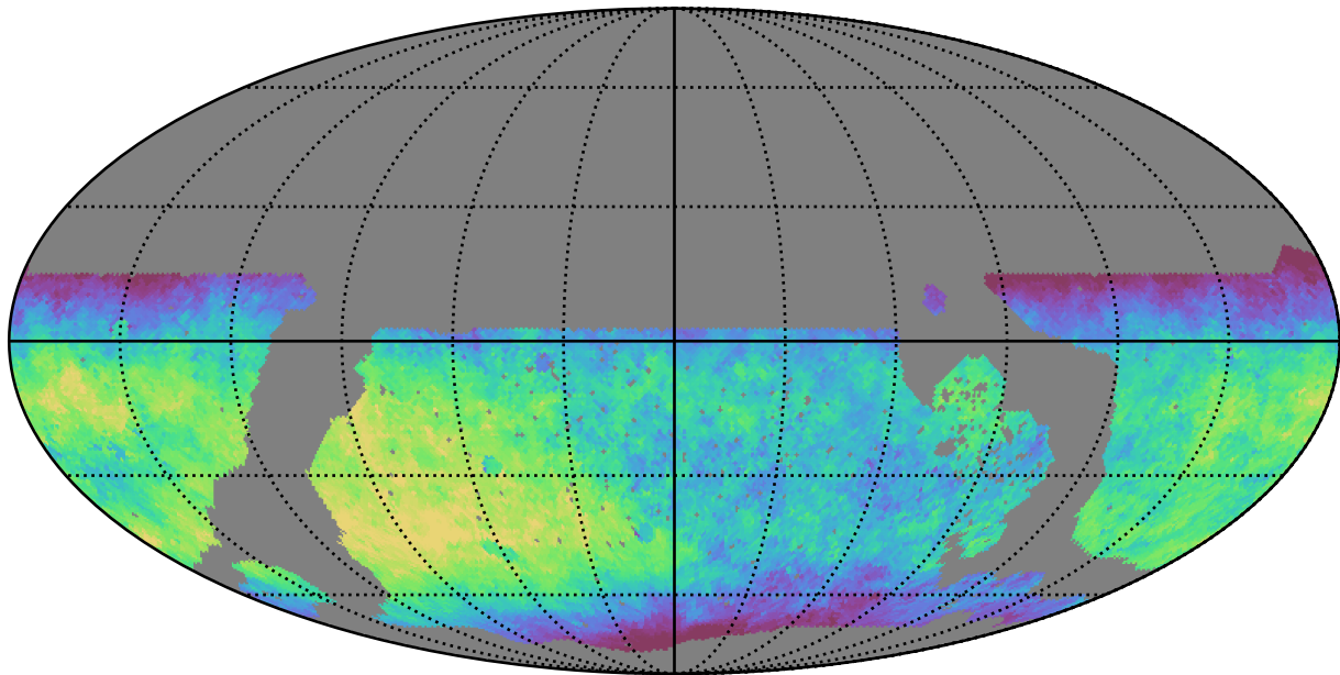
noroll_v3.4_10yrs WFD z band: Median fiveSigmaDepth
