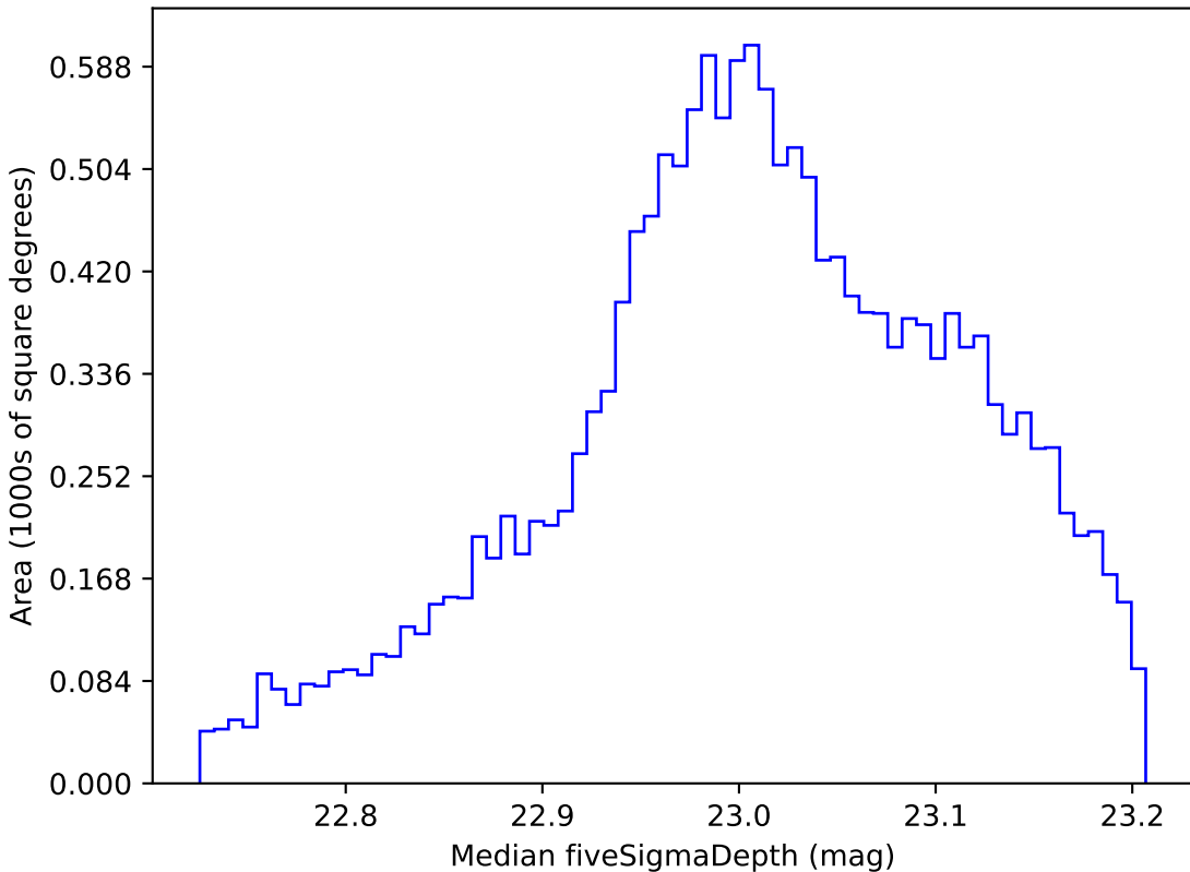
noroll_v3.4_10yrs WFD z band: Median fiveSigmaDepth
