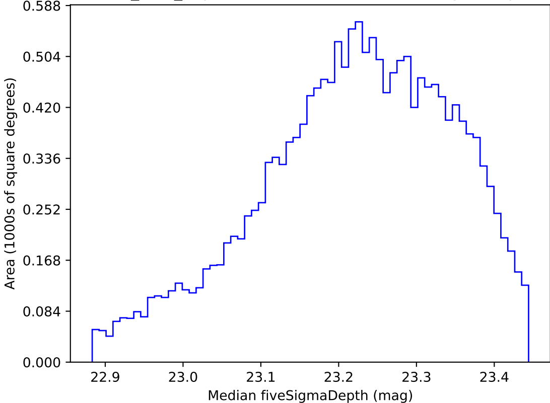
noroll_v3.4_10yrs WFD u band: Median fiveSigmaDepth
