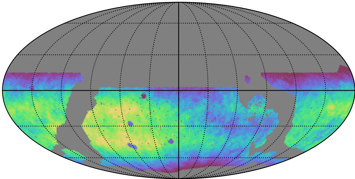
noroll_v3.4_10yrs WFD r band: Median fiveSigmaDepth
