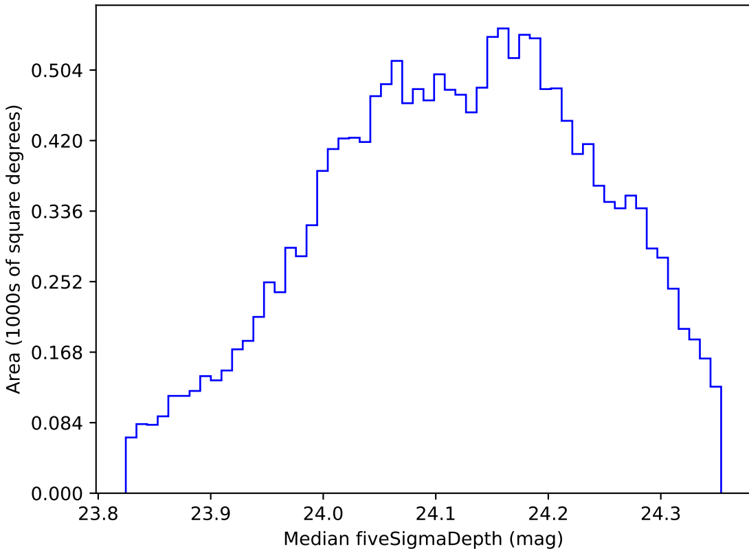
noroll_v3.4_10yrs WFD r band: Median fiveSigmaDepth
