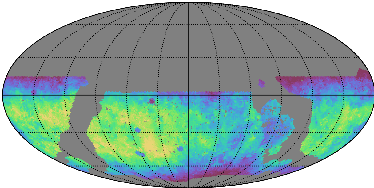
noroll_v3.4_10yrs WFD g band: Median fiveSigmaDepth
