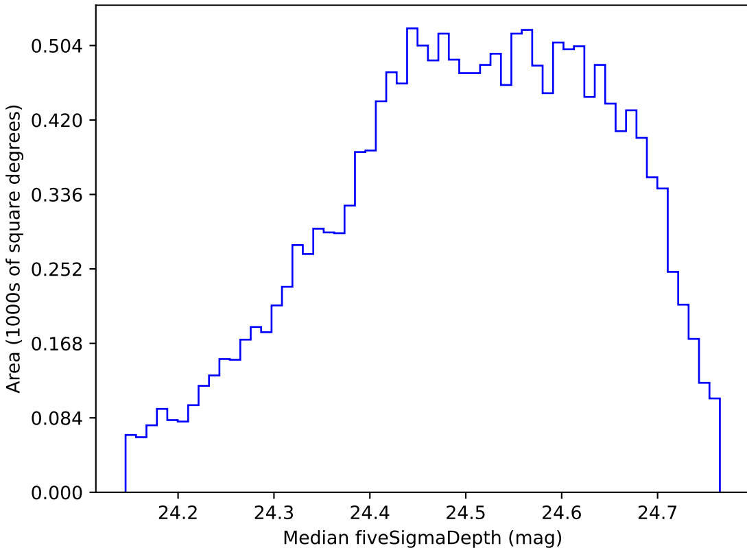
noroll_v3.4_10yrs WFD g band: Median fiveSigmaDepth
