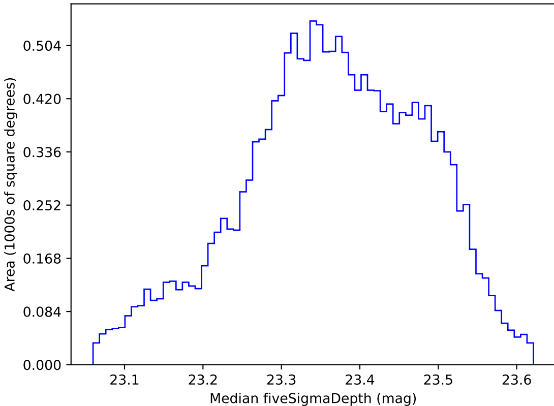
noroll_v3.4_10yrs WFD all bands: Median fiveSigmaDepth
