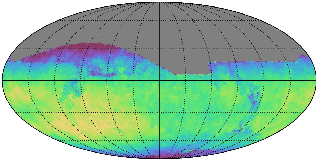
noroll_v3.4_10yrs All sky z band: Median fiveSigmaDepth
