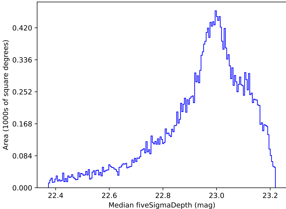
noroll_v3.4_10yrs All sky z band: Median fiveSigmaDepth
