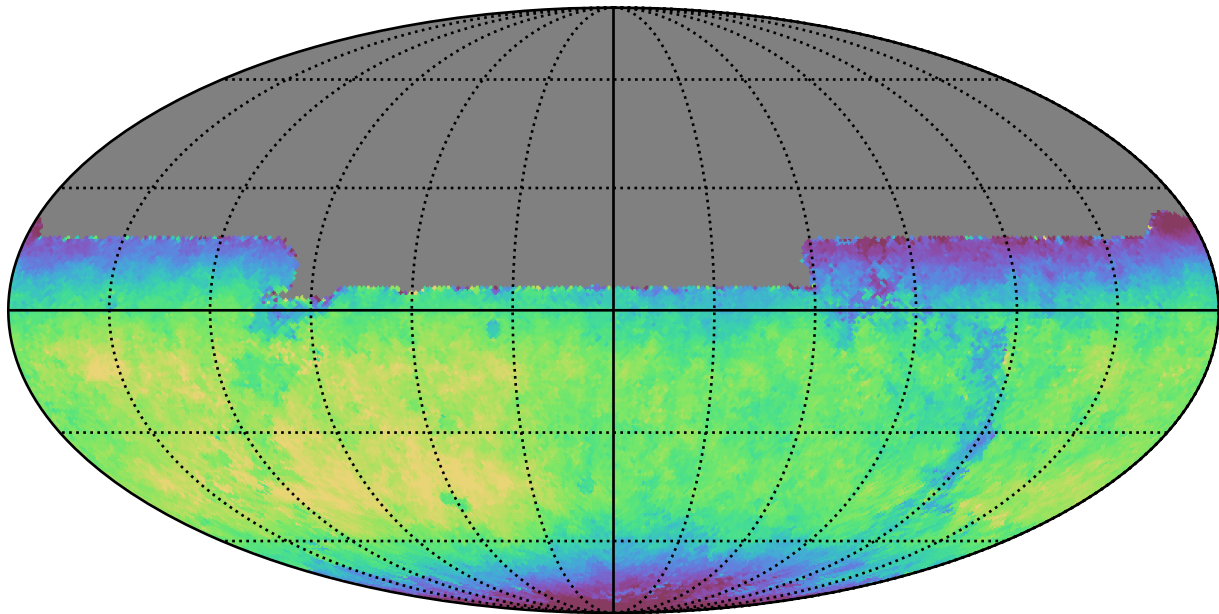
noroll_v3.4_10yrs All sky y band: Median fiveSigmaDepth
