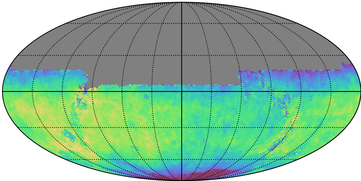
noroll_v3.4_10yrs All sky u band: Median fiveSigmaDepth
