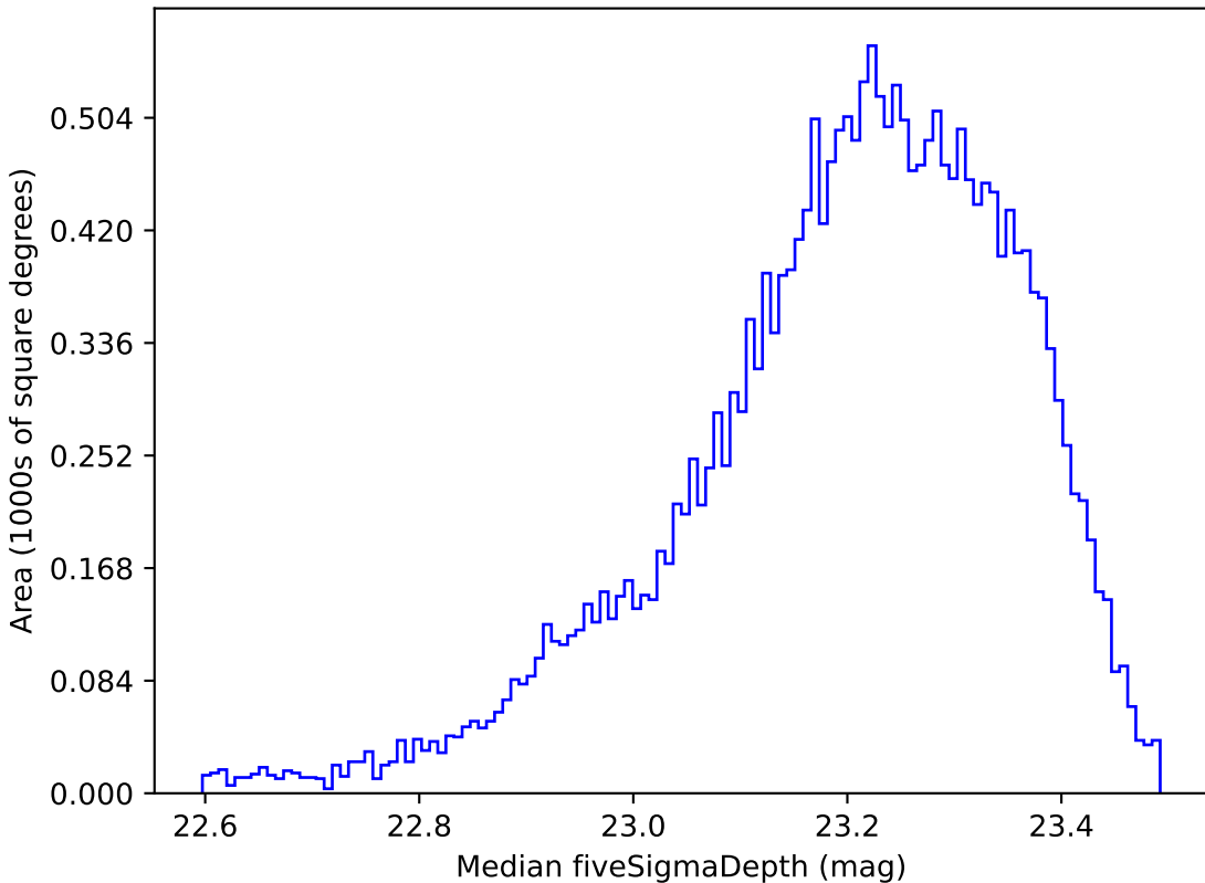
noroll_v3.4_10yrs All sky u band: Median fiveSigmaDepth
