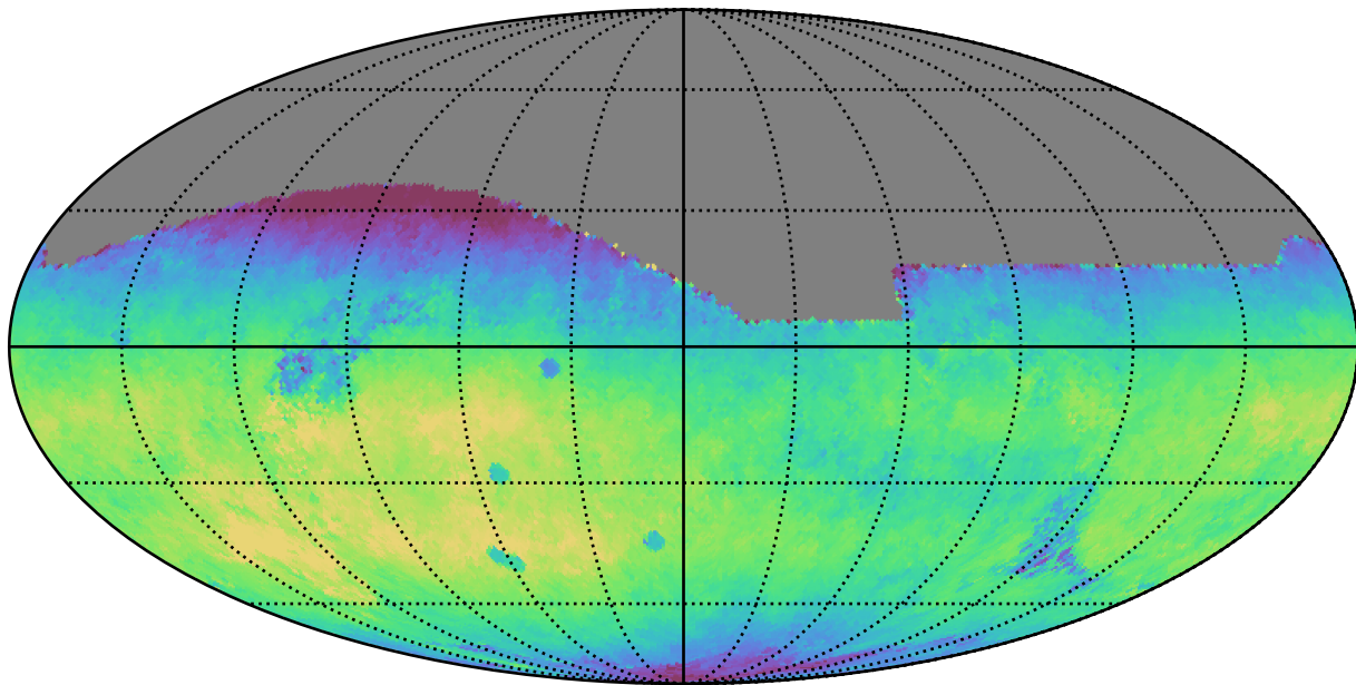
noroll_v3.4_10yrs All sky r band: Median fiveSigmaDepth
