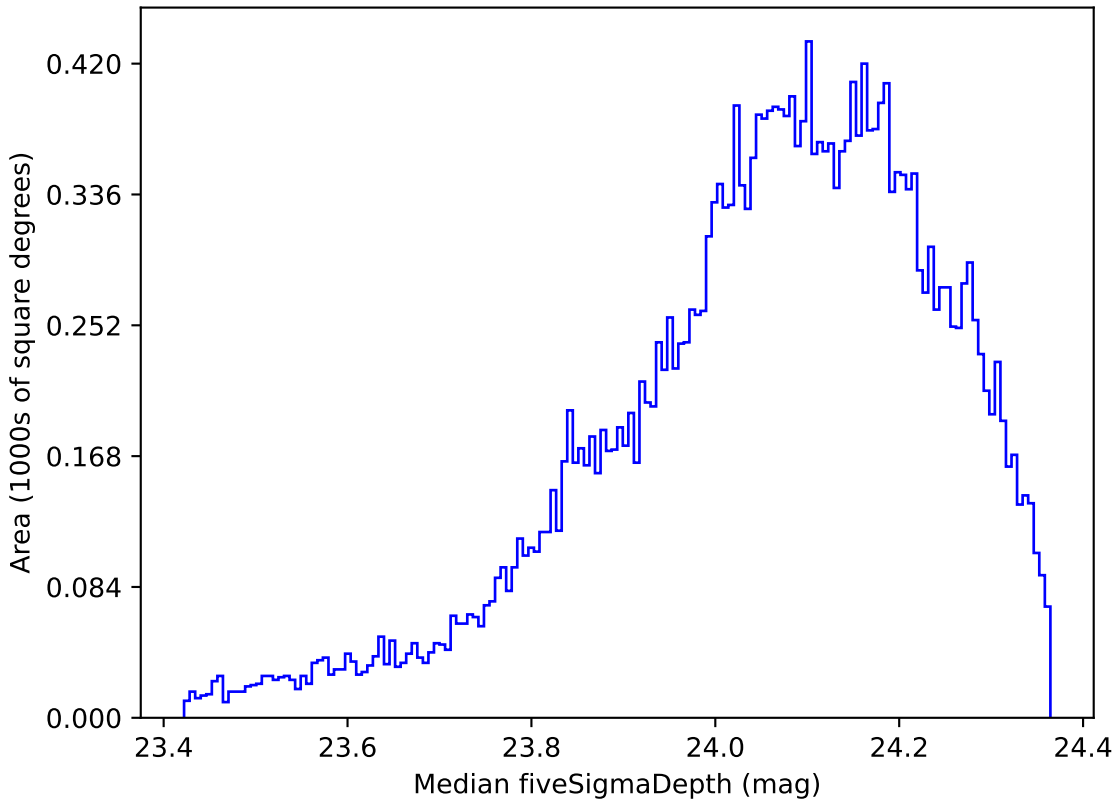
noroll_v3.4_10yrs All sky r band: Median fiveSigmaDepth
