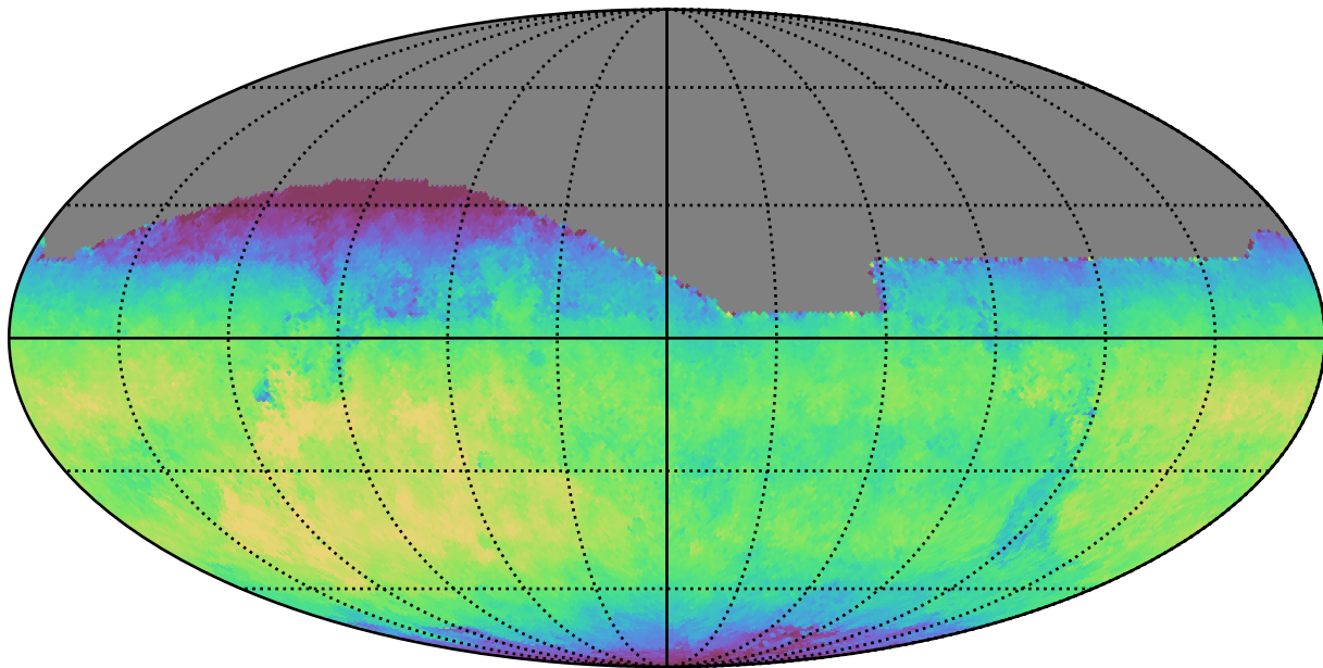
noroll_v3.4_10yrs All sky i band: Median fiveSigmaDepth
