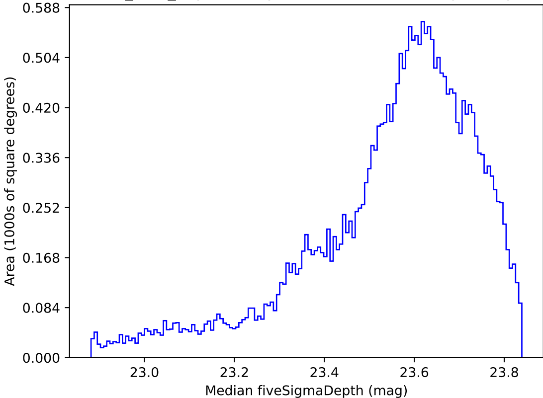
noroll_v3.4_10yrs All sky i band: Median fiveSigmaDepth
