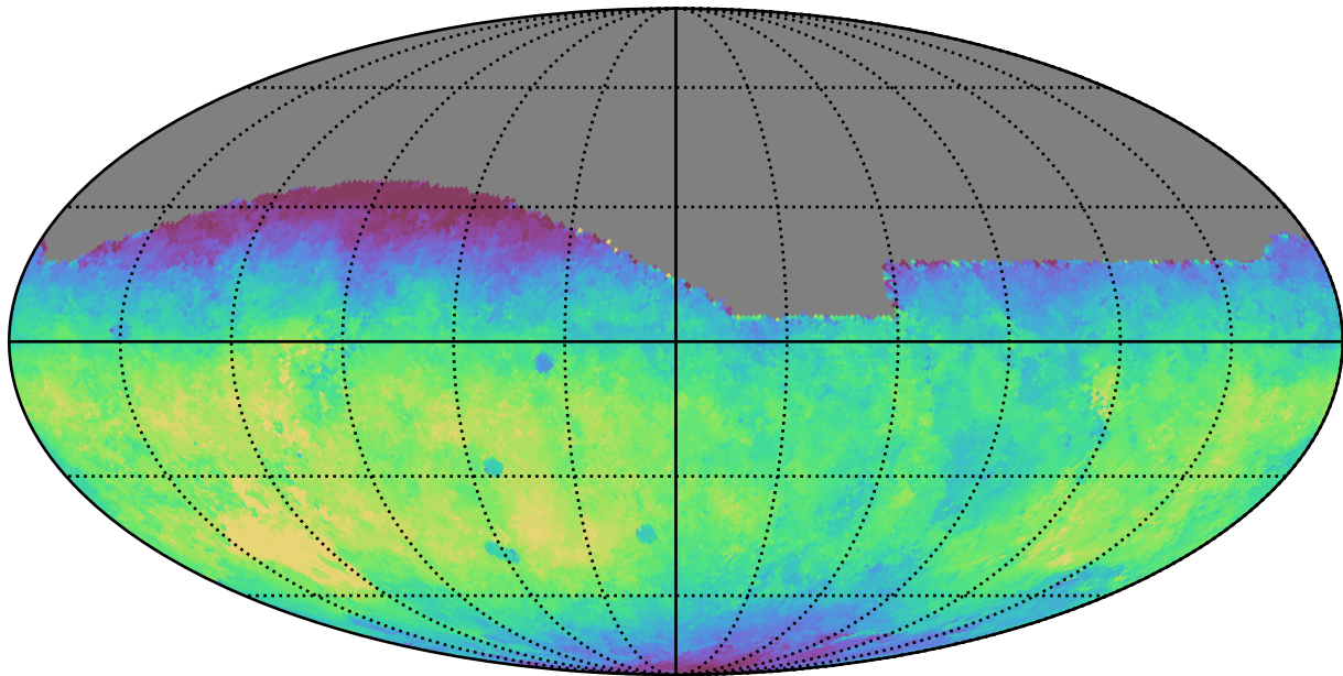
noroll_v3.4_10yrs All sky g band: Median fiveSigmaDepth
