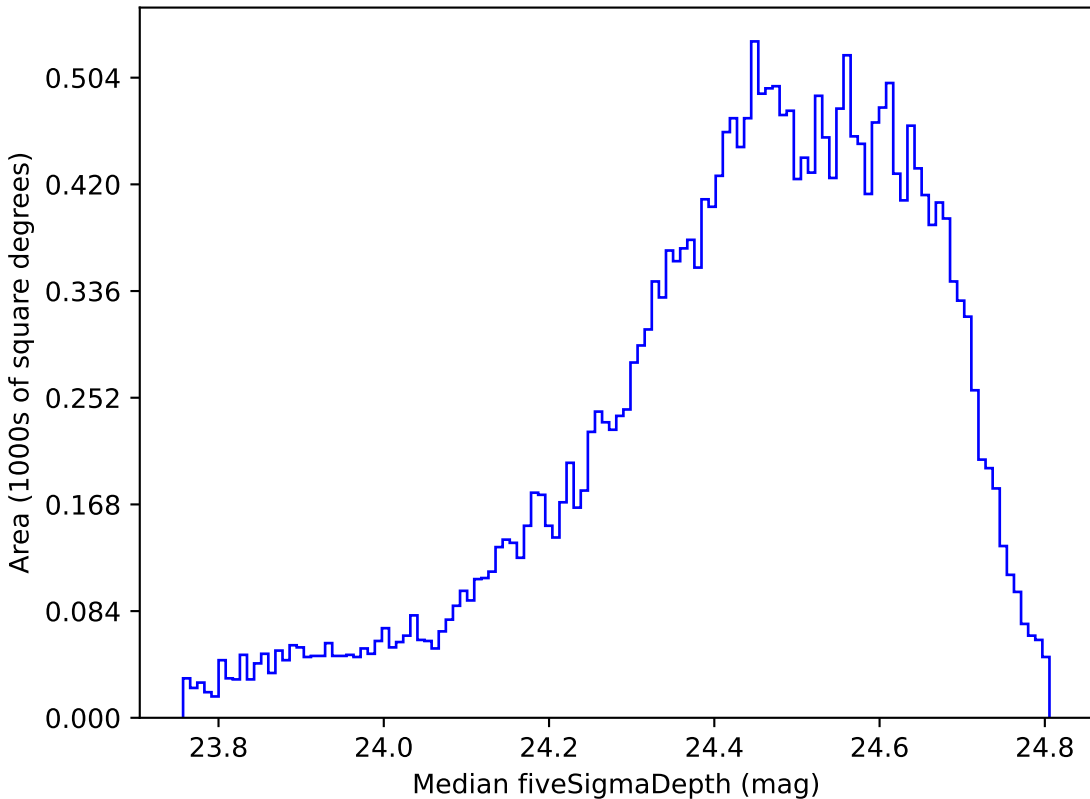
noroll_v3.4_10yrs All sky g band: Median fiveSigmaDepth
