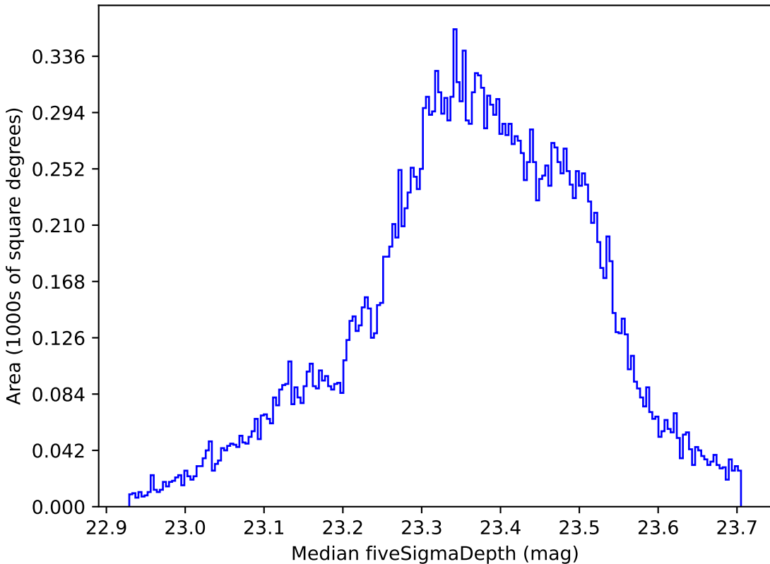
noroll_v3.4_10yrs All sky all bands: Median fiveSigmaDepth
