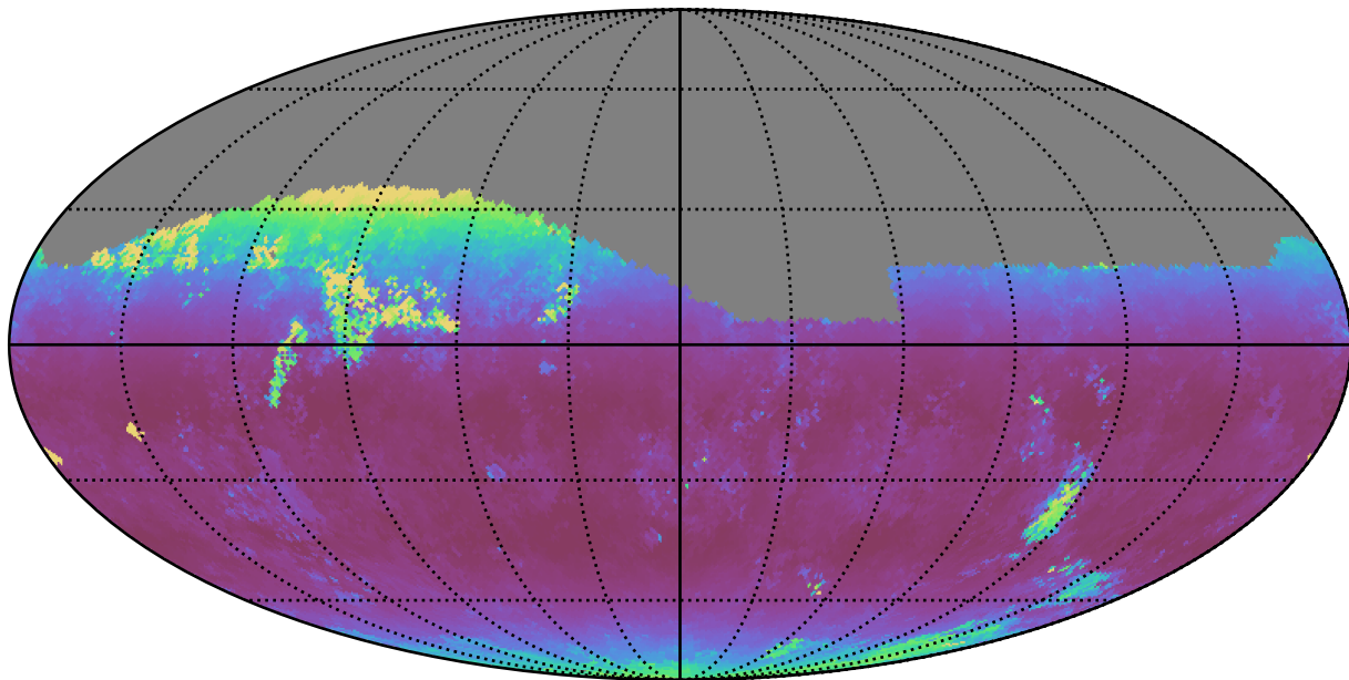
noroll_v3.4_10yrs Yr 1 z band: Median airmass
