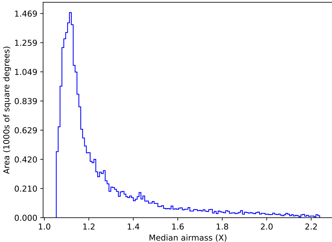
noroll_v3.4_10yrs Yr 1 z band: Median airmass
