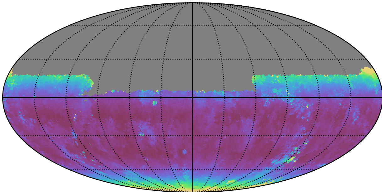
noroll_v3.4_10yrs Yr 1 y band: Median airmass
