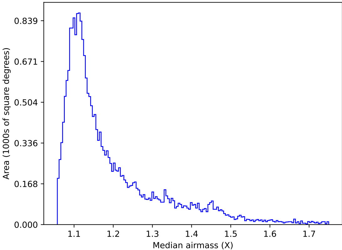
noroll_v3.4_10yrs Yr 1 y band: Median airmass
