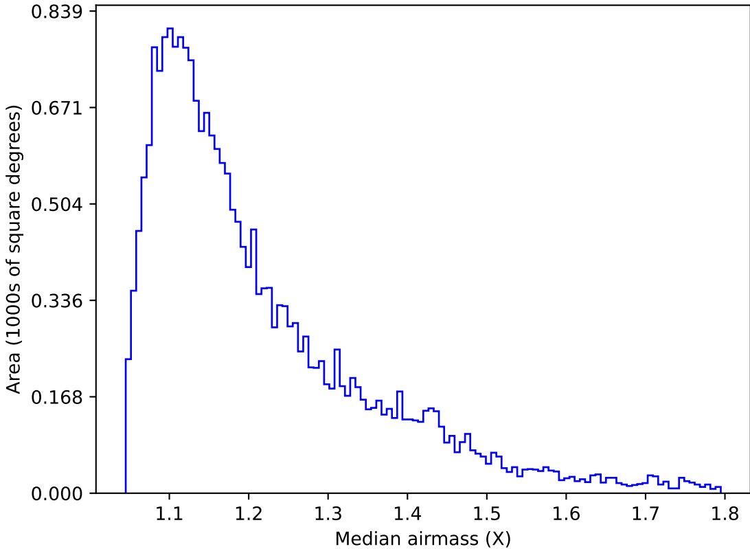
noroll_v3.4_10yrs Yr 1 u band: Median airmass
