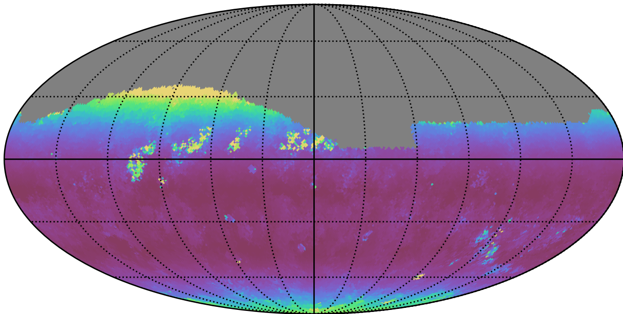
noroll_v3.4_10yrs Yr 1 r band: Median airmass
