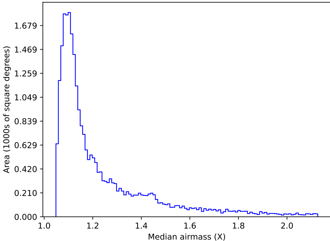
noroll_v3.4_10yrs Yr 1 r band: Median airmass
