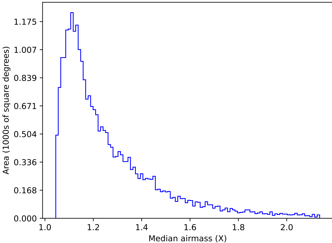
noroll_v3.4_10yrs Yr 1 g band: Median airmass
