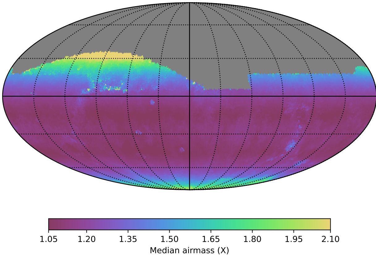
noroll_v3.4_10yrs Yr 1 all bands: Median airmass
