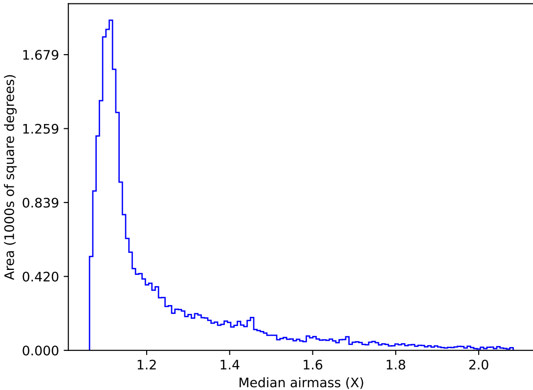
noroll_v3.4_10yrs Yr 1 all bands: Median airmass
