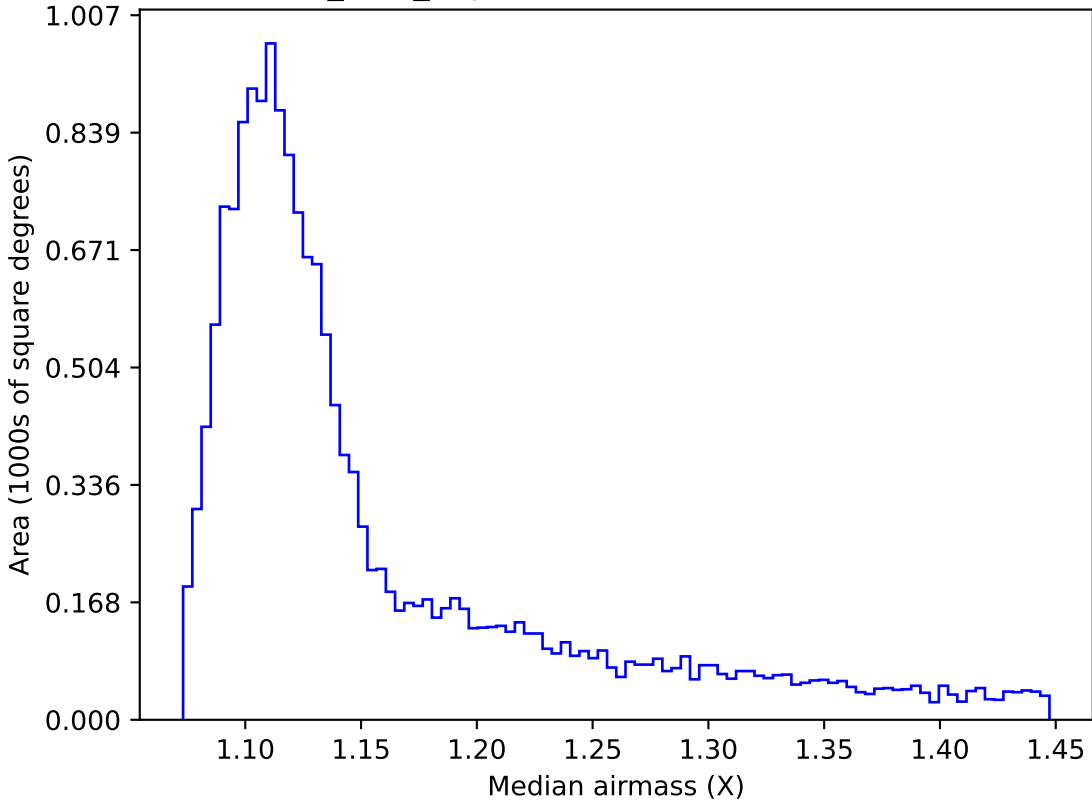
noroll_v3.4_10yrs WFD z band: Median airmass
