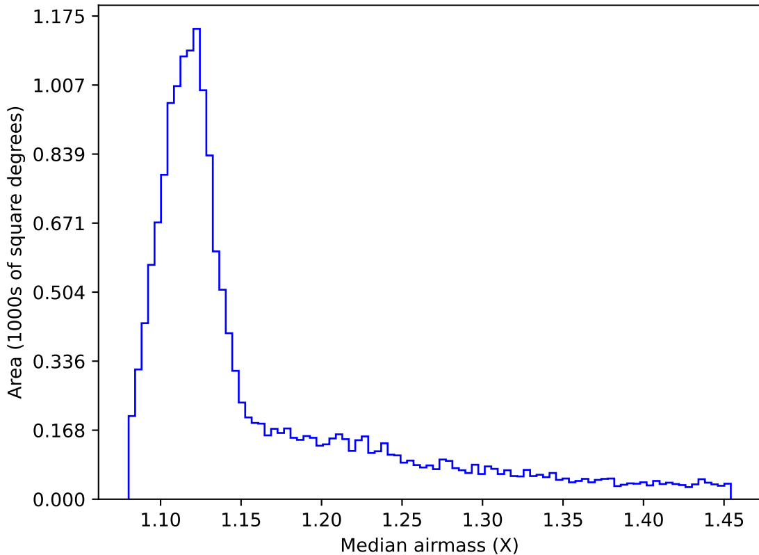
noroll_v3.4_10yrs WFD y band: Median airmass
