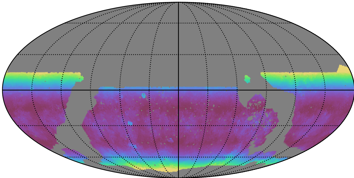
noroll_v3.4_10yrs WFD u band: Median airmass
