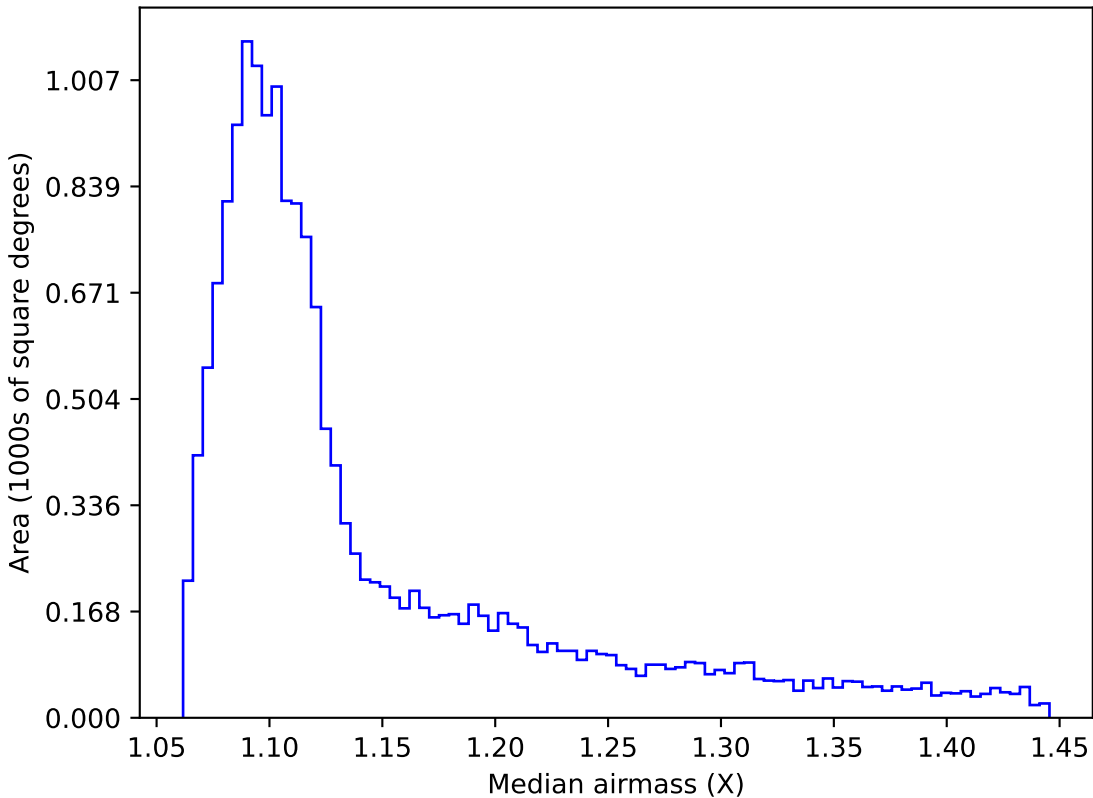
noroll_v3.4_10yrs WFD u band: Median airmass
