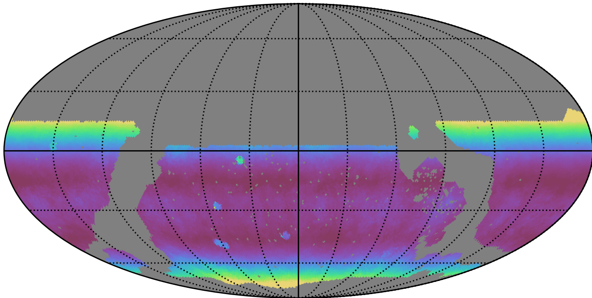
noroll_v3.4_10yrs WFD r band: Median airmass
