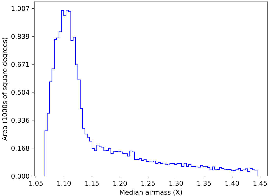
noroll_v3.4_10yrs WFD i band: Median airmass
