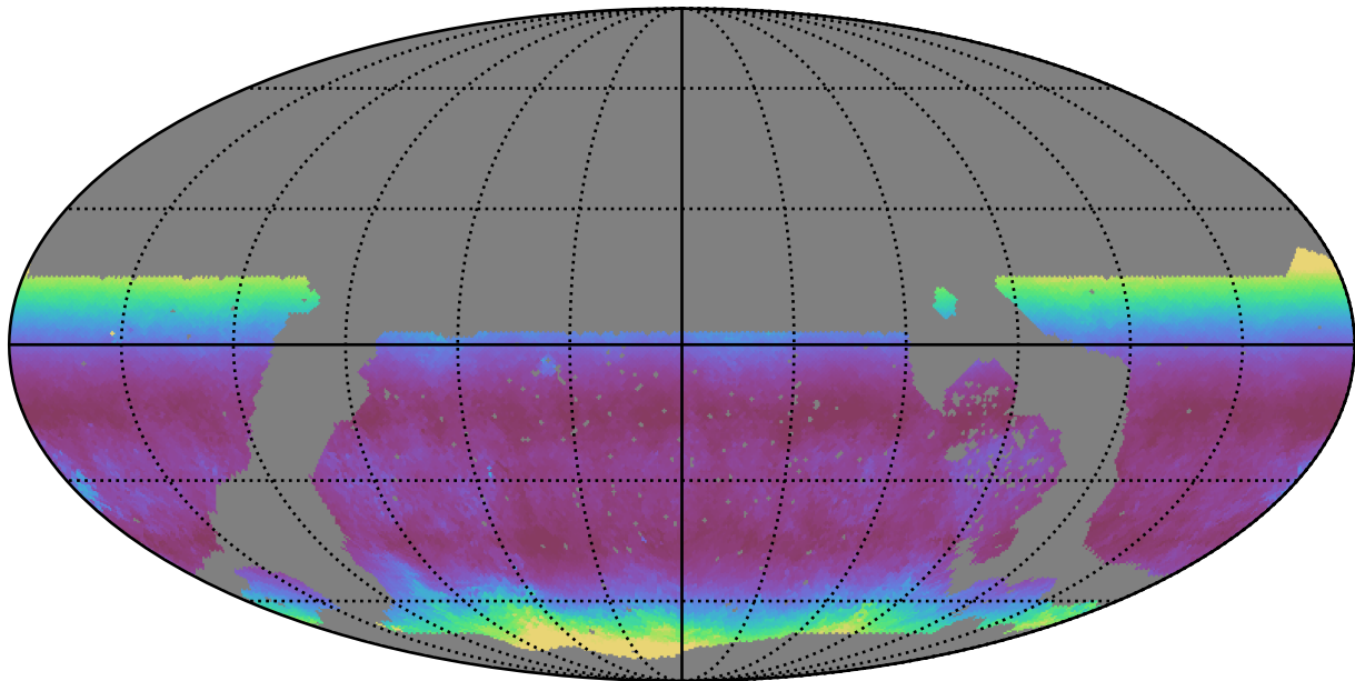
noroll_v3.4_10yrs WFD g band: Median airmass
