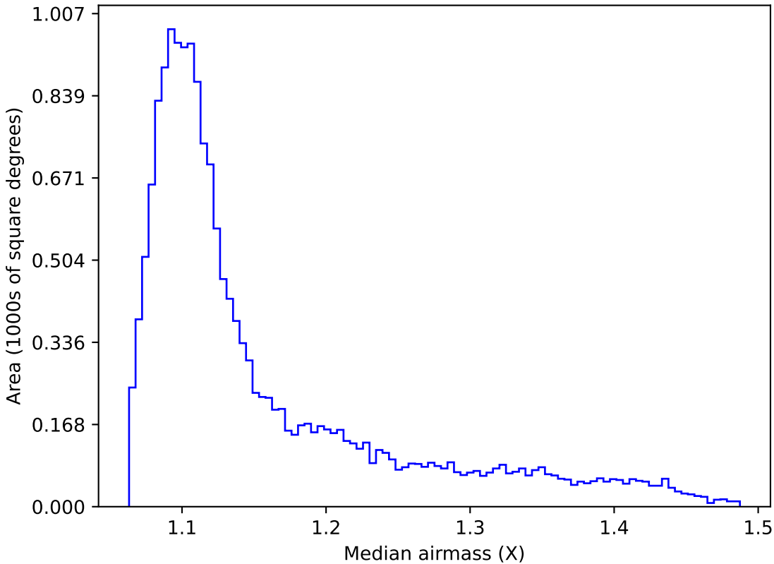
noroll_v3.4_10yrs WFD g band: Median airmass
