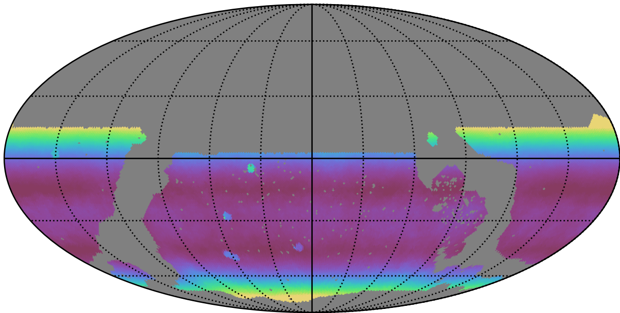
noroll_v3.4_10yrs WFD all bands: Median airmass
