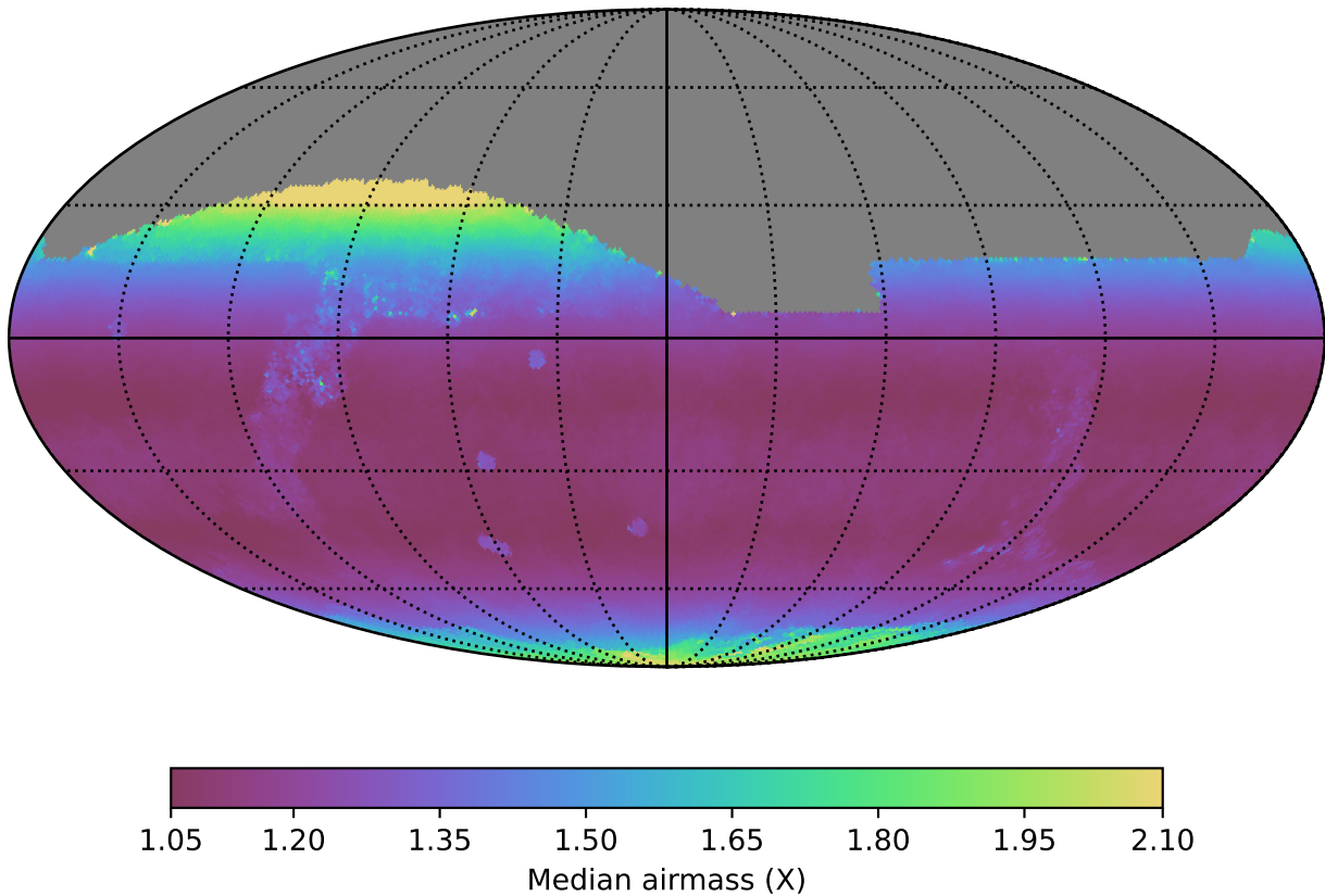
noroll_v3.4_10yrs All sky z band: Median airmass
