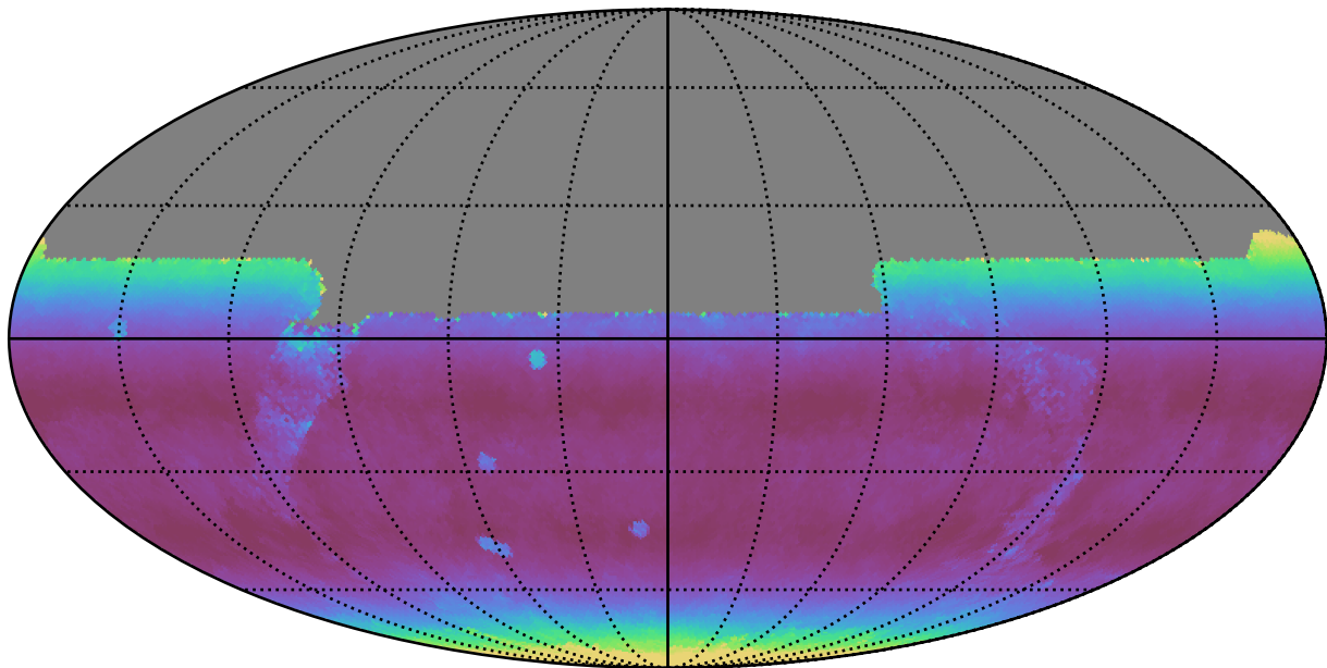
noroll_v3.4_10yrs All sky y band: Median airmass
