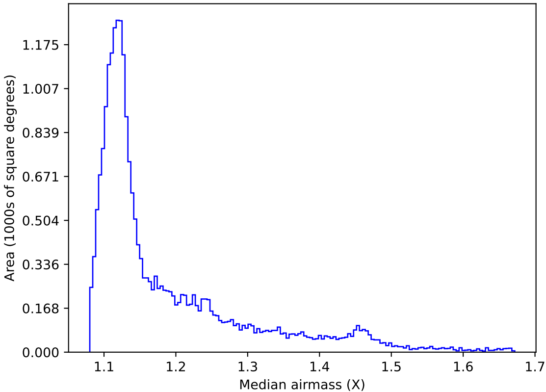
noroll_v3.4_10yrs All sky y band: Median airmass
