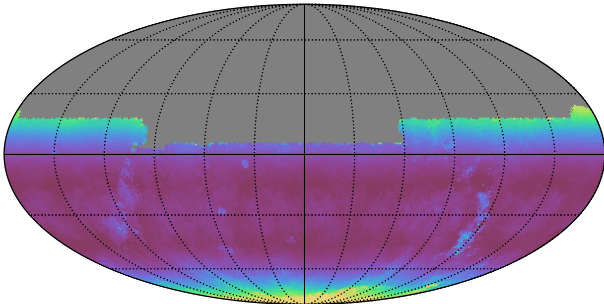
noroll_v3.4_10yrs All sky u band: Median airmass
