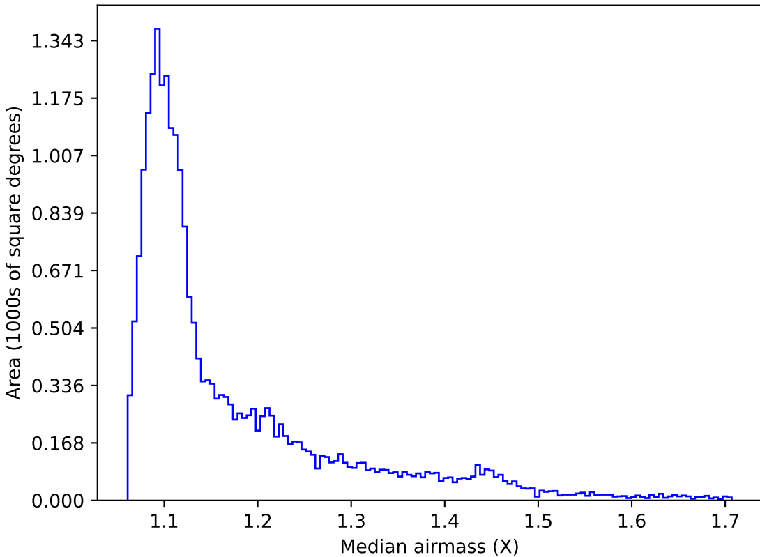
noroll_v3.4_10yrs All sky u band: Median airmass
