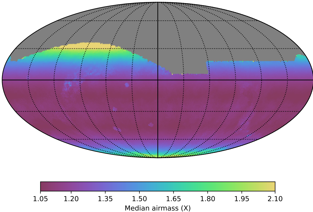
noroll_v3.4_10yrs All sky r band: Median airmass
