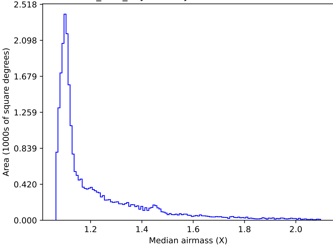
noroll_v3.4_10yrs All sky r band: Median airmass
